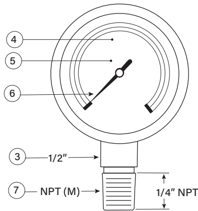
THREAD CONNECTION
