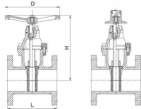
Size 2"-12"
