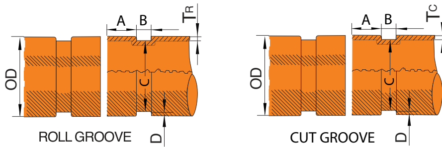
PIPE GROOVING SPECIFICATIONS (AWWA C606)
