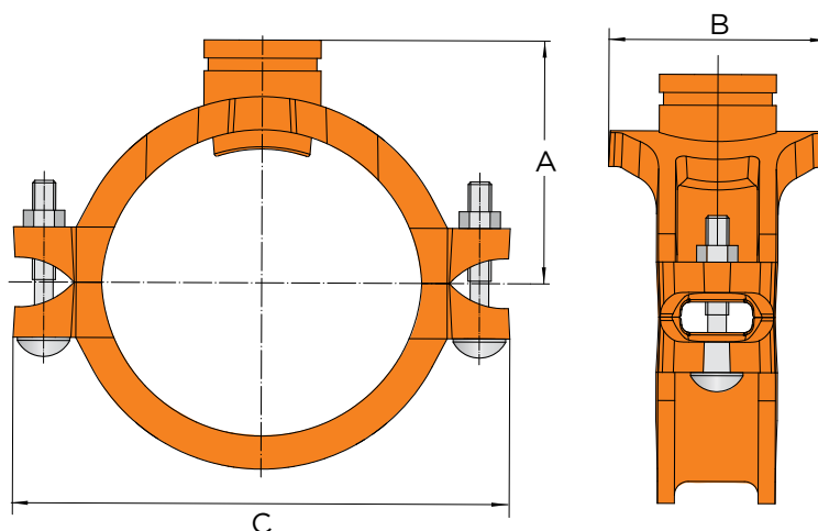
MECHANICAL TEE - GROOVED STYLE 15
