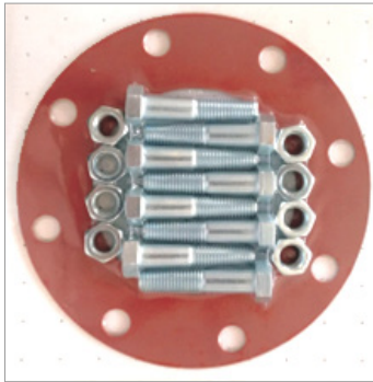
Both ring and full face gaskets are available for ASTM CL 150 and 300 Flanges
