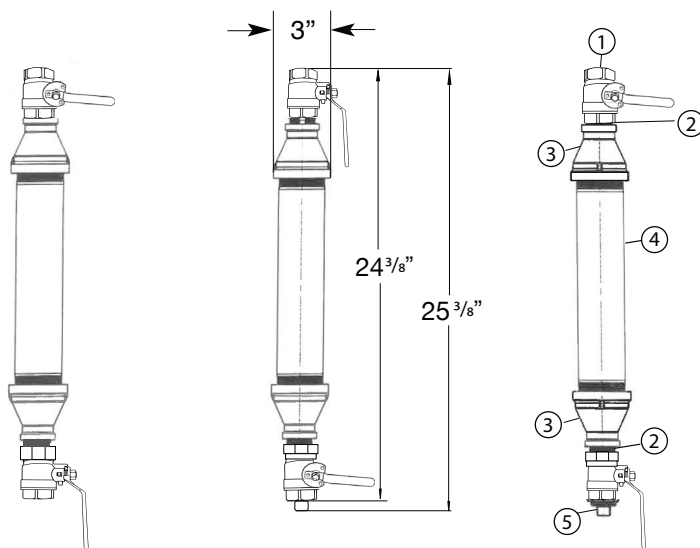
DRAIN MODE
